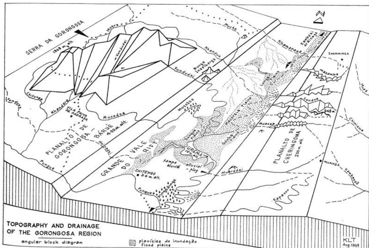
Figure 1. Block diagram showing landscape units of the Greater Gorongosa region and drainage pathways to the Rift Valley floor (from Tinley 1977).
