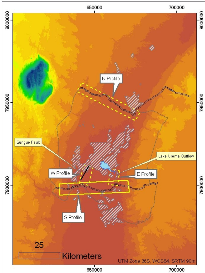
Figure 7. Proposed resistivity transect along the Chitengo-Muanza Road, using groundbased multi-electrode resistivity surveying (solid yellow box). Based on results, additional north-south and east-west transects may be planned (dashed yellow boxes).
