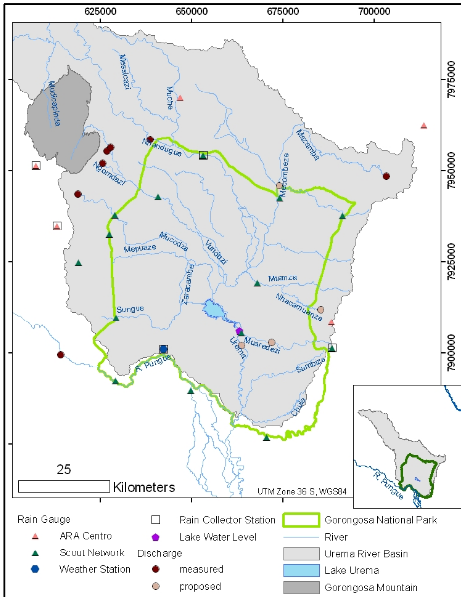
Figure 6. Current and proposed hydrometric monitoring stations around Gorongosa NP.
