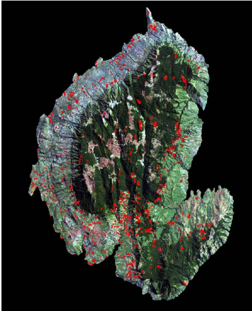
Figure 4. Afromontane forest and wet miombo woodland loss (areas shown in red) on Gorongosa Mountain above 700 meters, 1992-2005 (Woods Hole Research Center 2006).
