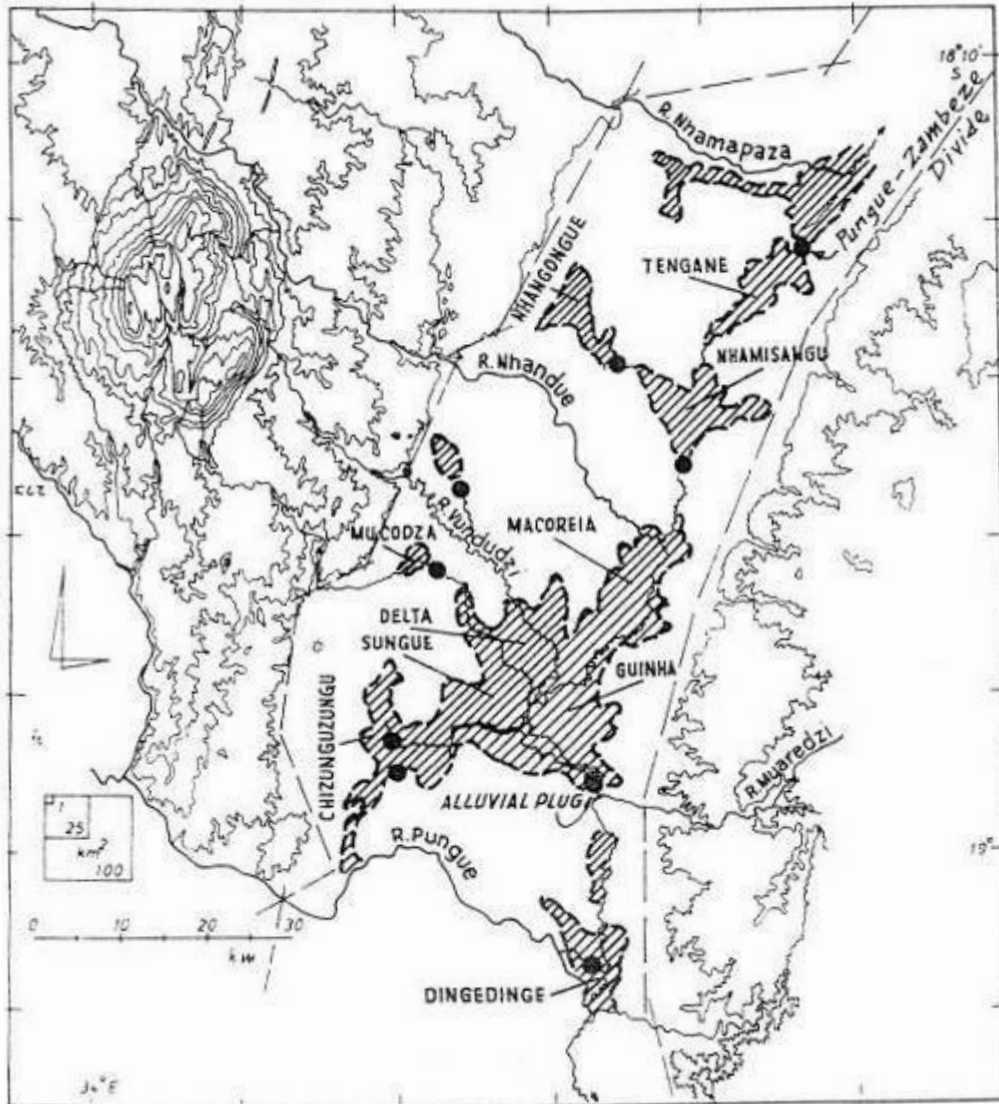
Figure 2. Floodplain swamps on the Rift Valley floor, in association with drainage from Gorongosa Mountain and the Rift Valley escarpment (from Tinley 1977).
